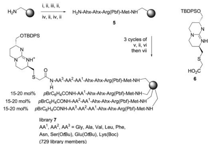
Scheme 3. i) Fmoc-Met, DIC, HOBT, DIPEA, DMF, 3 h; ii) 20% piperidine/DMF, 20 min; iii) Fmoc-Arg(Pbf), DIC, HOBT, DIPEA, DMF, 3 h; iv) Fmoc-Ahx, DIC, HOBT, DIPEA, DMF, 3 h; v) Fmoc-AA, DIC, HOBT, DIPEA, DMF, 3 h; vi) p\text{-BrC}_6\text{H}_4\text{COOH} (15–20 mol-%), DIC, HOBT, DIPEA, DMF, 18 h; vii) 6 , DIC, HOBT, DIPEA, DMF, 3 h.
