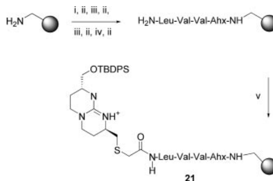
Scheme 6. i) Fmoc-Ahx, DIC, HOBT, DIPEA, DMF, 3 h; ii) 20% piperidine/DMF, 20 min; iii) Fmoc-Val, DIC, HOBT, DIPEA, DMF, 3 h; iv) Fmoc-Leu, DIC, HOBT, DIPEA, DMF, 3 h; v) 6 , EDC, HOBT, DIPEA, DMAP, DMF, 1 h.
