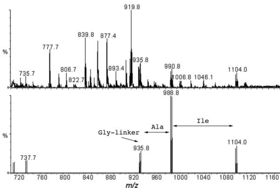
Figure 1. Mass spectra of a sample from a single cleaved bead of 3 a) raw data, b) processed to identify Br-isotope patterns.
