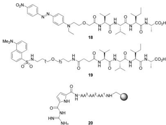
Figure 2. Dye-labelled peptide 18 used in screening experiments with library 7 , and dye-labelled peptide 19 used by Schmuck in screening experiment with library 20 .
