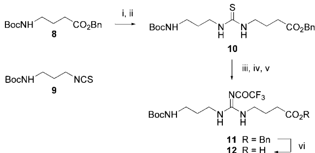
Scheme 4. i) \text{CF}_3\text{CO}_2\text{H} , DCM; ii) 9 , \text{Et}_3\text{N} , DCM/MeOH, 18 h; iii) MeI, acetone, 1 h; iv) \text{NH}_4\text{PF}_6 , DCM/MeOH, 18 h; v) \text{F}_3\text{CCONH}_2 , DBU, toluene/ \text{CHCl}_3 , 2 h; vi) \text{H}_2 , Pd/C, EtOAc, 3 h.
